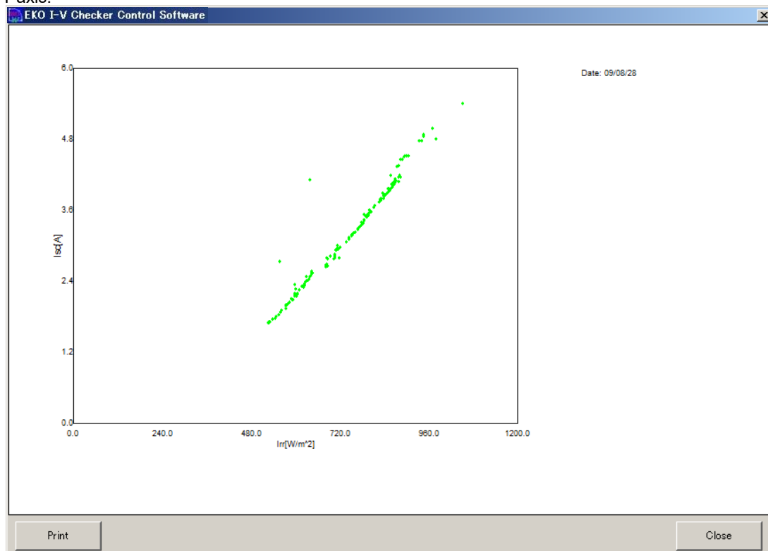
Figure 9-3-25. Irradiance vs. Short Circuit Current Graph
