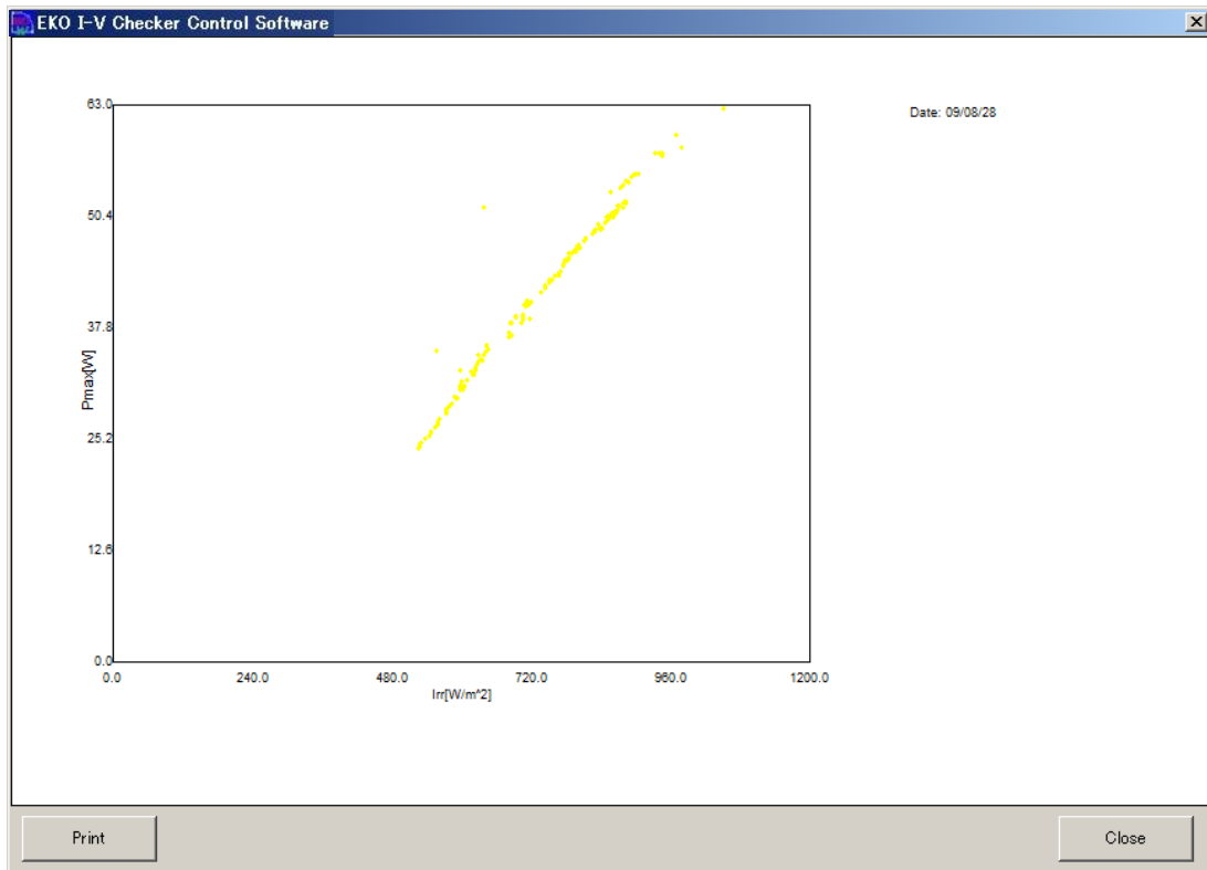
Figure 9-3-26. Irradiance vs. Maximum Power Graph
