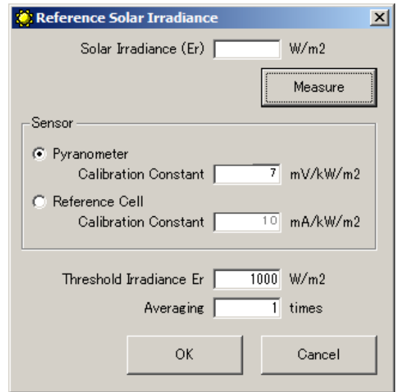
Figure 9-3-5. Reference Solar Irradiance Setting
