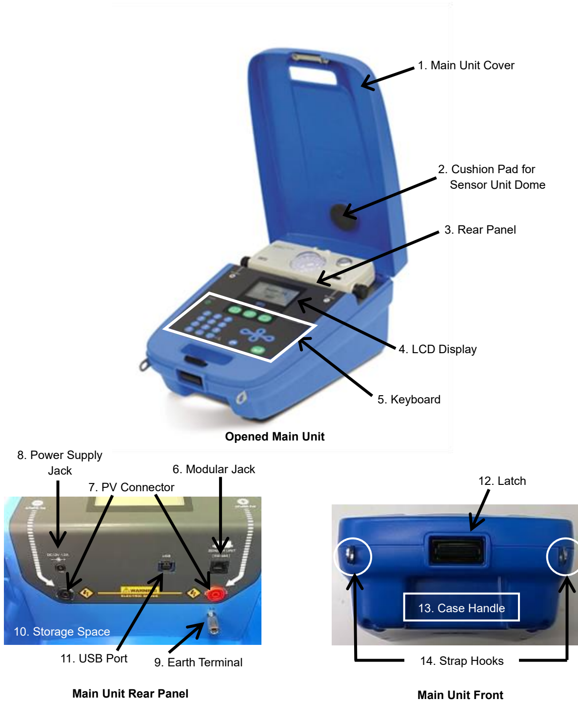
Figure 5-1. Main Unit Parts Name and Functions
