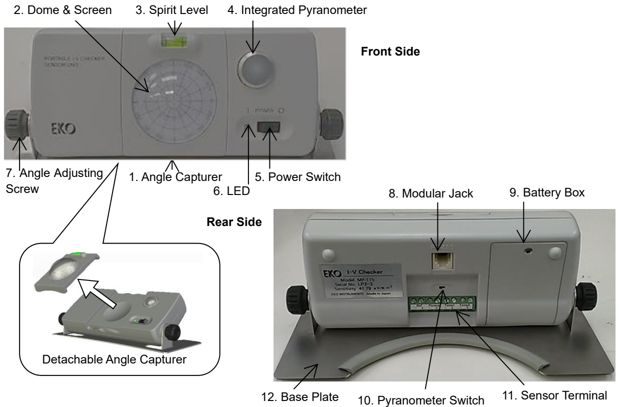
Figure 5-2. Sensor Unit Parts Name and Function
