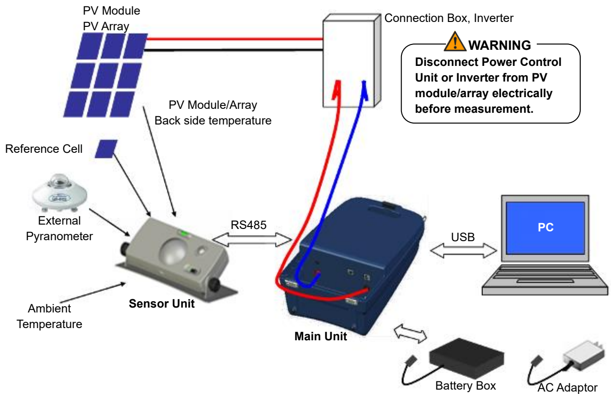
Figure 5-5. System Configuration
