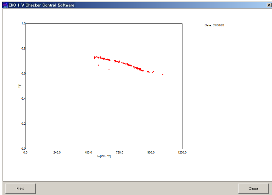
Figure 9-3-27. Irradiance vs. Fill Factor Graph
