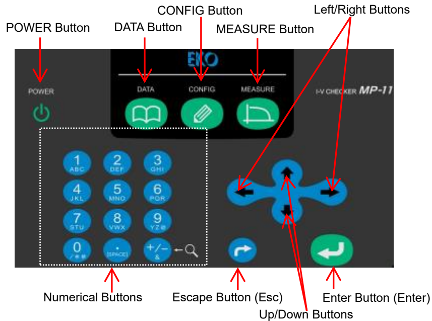
Figure 8-1. Operation Panel
